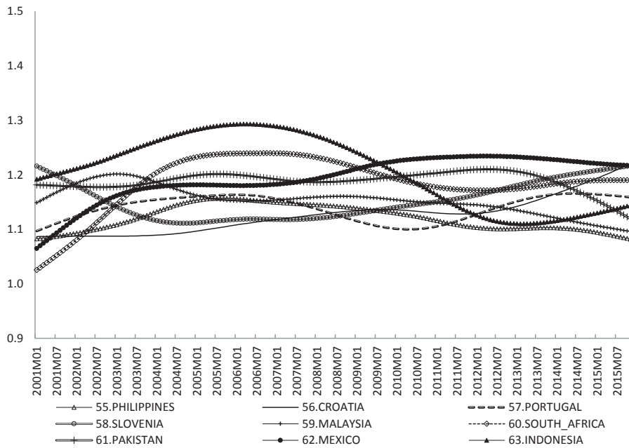
Fig. 2g. Relative transition paths for countries 55–63 (2001M1-2015M12).
