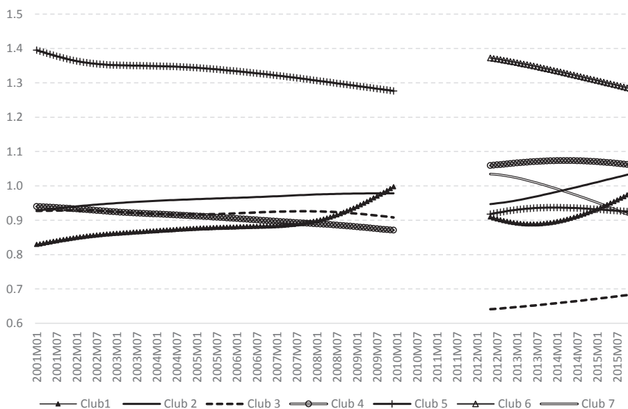
Fig. 4d. Relative transition paths across clubs (3rd breakpoint-homogenous group).
