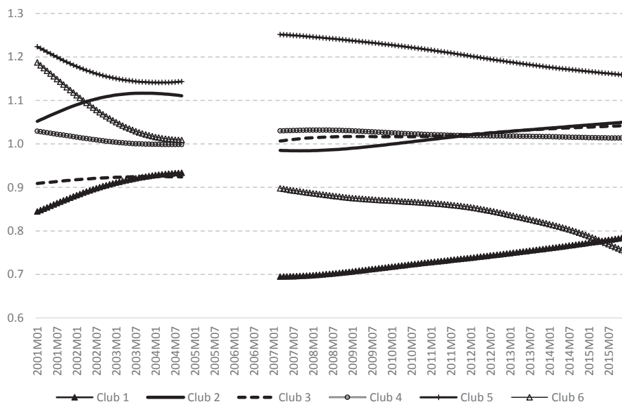
Fig. 4b. Relative transition paths across clubs (1st breakpoint-homogenous group).
